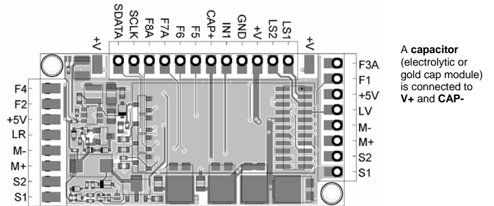
ADAMTC – without low-voltage supply ADAMTC15 or ADAMTC50 – with 1.5 or 5.0 V supply
